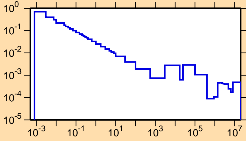
\sigma vs. E for ^{50}\text{Ti}(n,\gamma)
