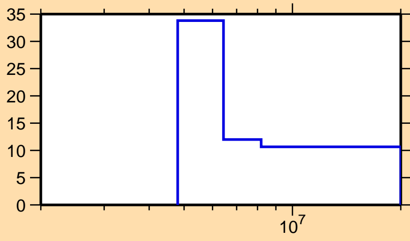
\Delta\sigma/\sigma vs. E for ^{50}\text{Ti}(n,n\text{cont.})
