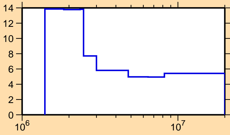
\Delta\sigma/\sigma vs. E for ^{50}\text{Ti}(n,\text{nonel.})
