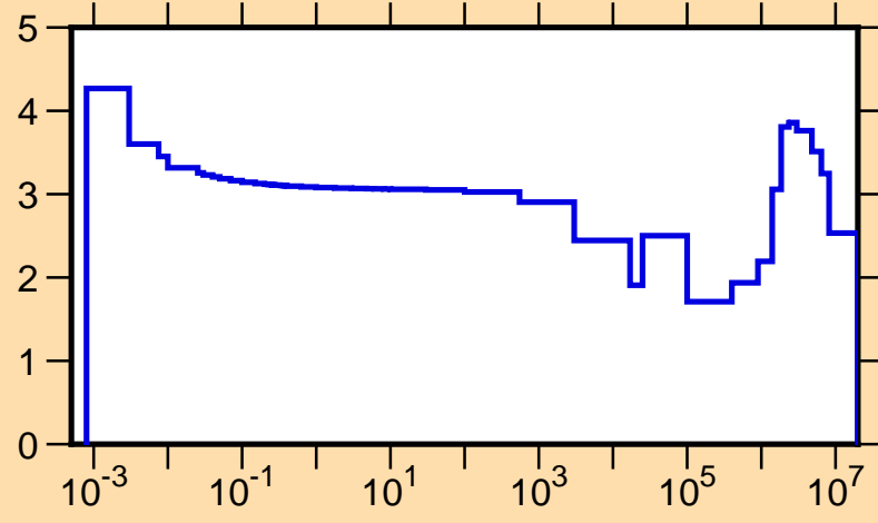
\sigma vs. E for ^{50}\text{Ti}(n,\text{tot.})
