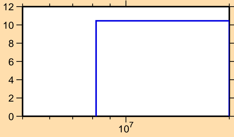
\Delta\sigma/\sigma vs. E for ^{50}\text{Ti}(n,2n)
