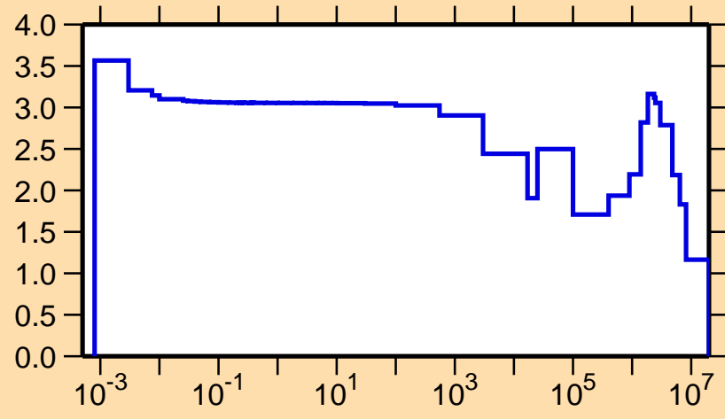
\sigma vs. E for ^{50}\text{Ti}(n,\text{el.})
