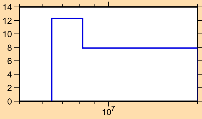
\Delta\sigma/\sigma vs. E for ^{50}\text{Ti}(n,\text{el.})
