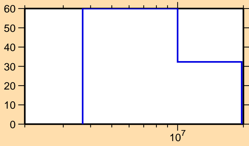
\Delta\sigma/\sigma vs. E for ^{51}\text{Ti}(n,\gamma)
