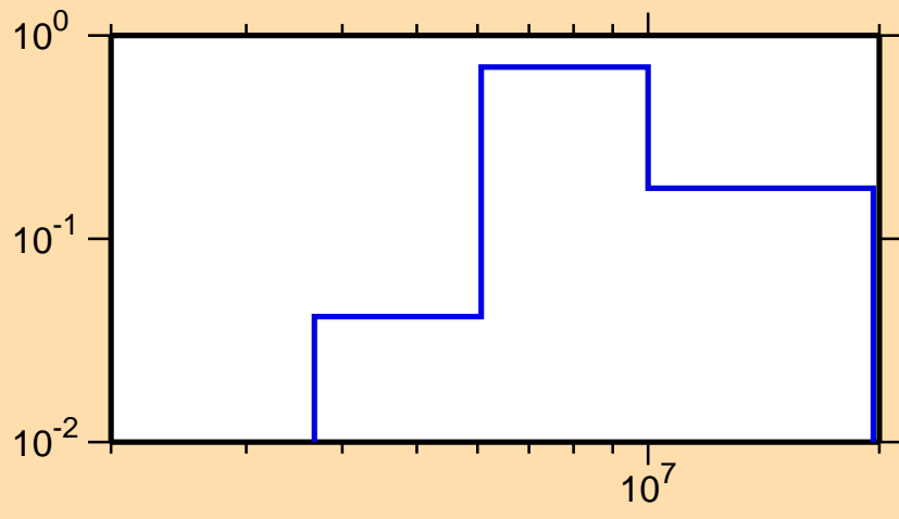
\sigma vs. E for ^{51}\text{Ti}(n,n\text{cont.})
