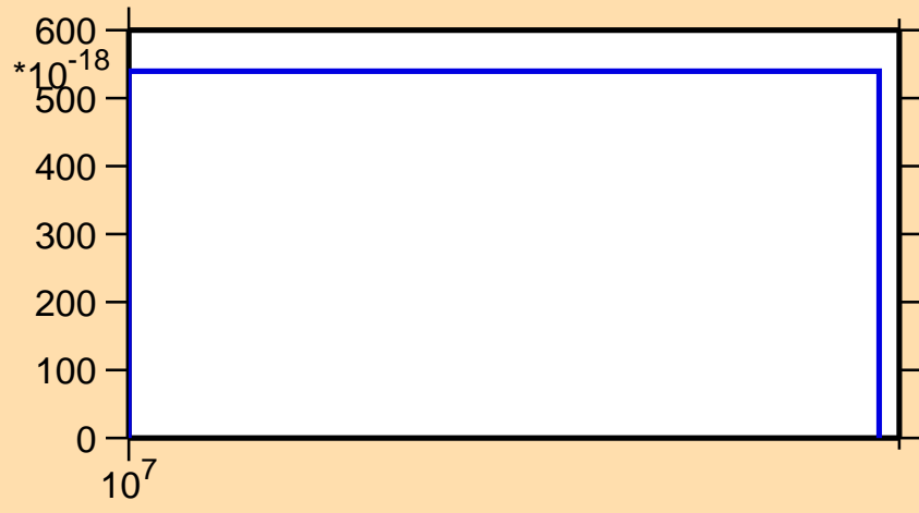
\sigma vs. E for ^{51}\text{Ti}(n,2n\alpha)
