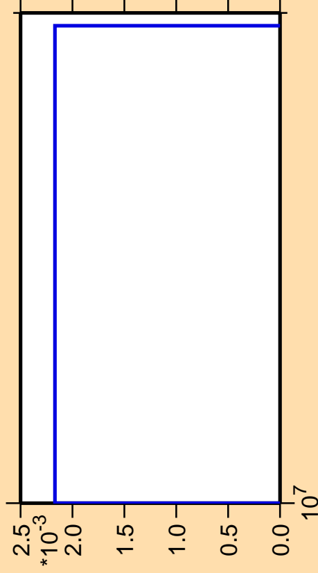
\Delta\sigma/\sigma vs. E for ^{51}\text{Ti}(n,2n\alpha)
