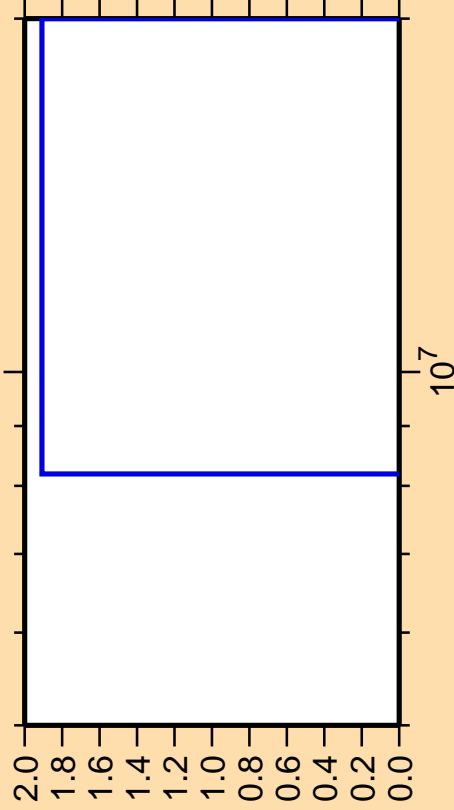
\Delta\sigma/\sigma vs. E for ^{51}\text{Ti}(n,2np)
