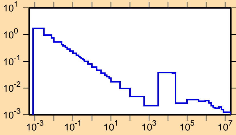
\sigma vs. E for ^{51}\text{Ti}(n,\gamma)
