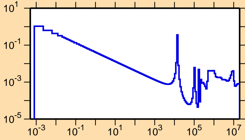
\sigma vs. E for ^{52}\text{Ti}(n,\gamma)
