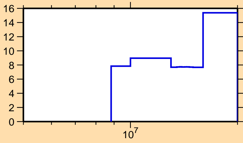
\Delta\sigma/\sigma vs. E for ^{52}\text{Ti}(n,2n)
