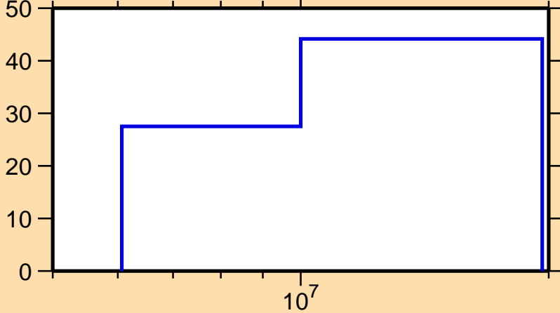
\Delta\sigma/\sigma vs. E for ^{52}\text{Ti}(n,n_1)
