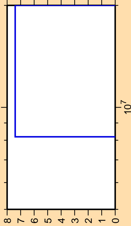
\Delta\sigma/\sigma vs. E for ^{52}\text{Ti}(n,2n)
