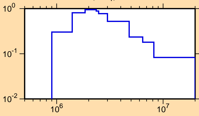
\sigma vs. E for ^{52}\text{Ti}(n,n_1)
