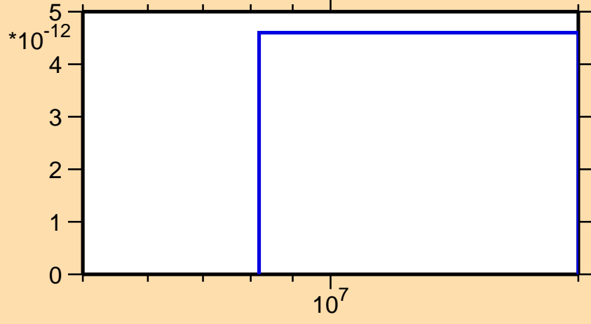
\sigma vs. E for ^{52}\text{Ti}(n,nd)
