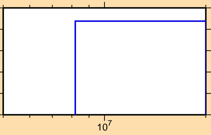
\sigma vs. E for ^{52}\text{Ti}(n,3n)
