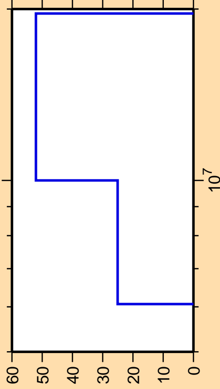
\Delta\sigma/\sigma vs. E for ^{53}\text{Ti}(n,n_1)
