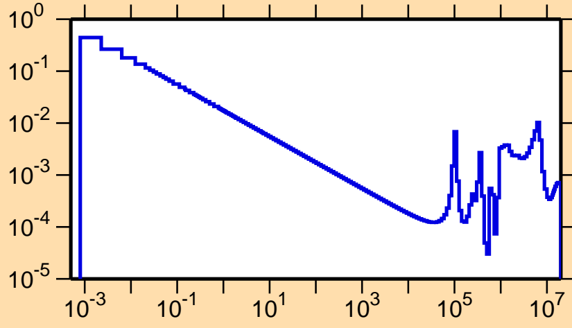
\sigma vs. E for ^{54}\text{Ti}(n,\gamma)
