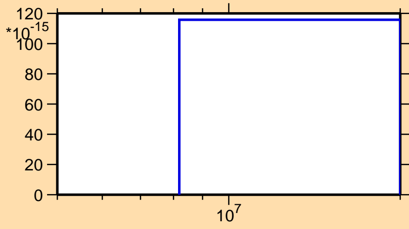
\sigma vs. E for ^{54}\text{Ti}(n,nd)
