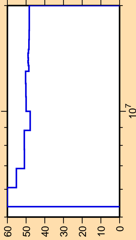
\Delta\sigma/\sigma vs. E for ^{55}\text{Ti}(n,n\text{cont.})
