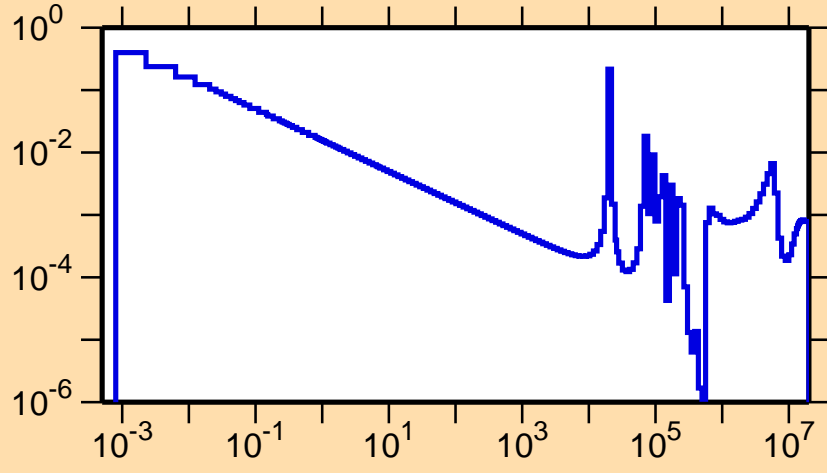
\sigma vs. E for ^{55}\text{Ti}(n,\gamma)
