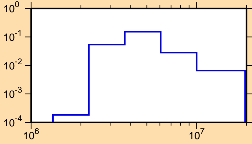
\sigma vs. E for ^{55}\text{Ti}(n,n_4)
