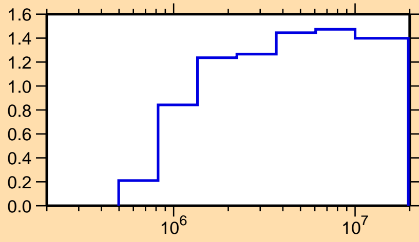
\sigma vs. E for ^{55}\text{Ti}(n,\text{nonel.})
