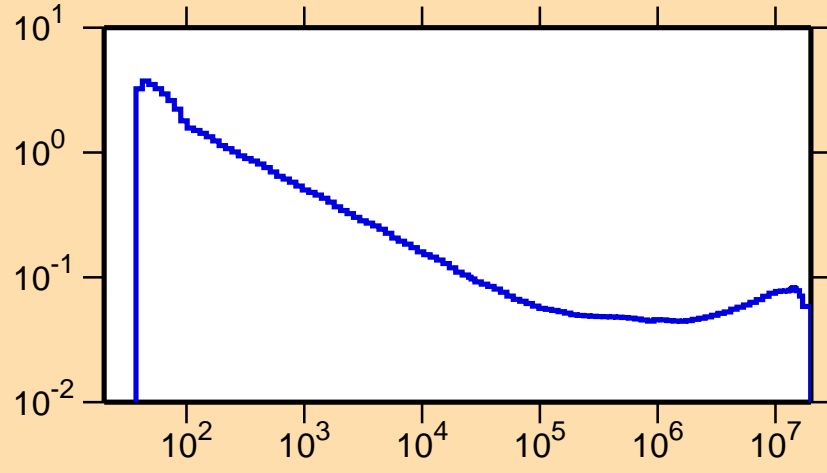
\sigma vs. E for ^{180}\text{Tl}(n,\alpha)
