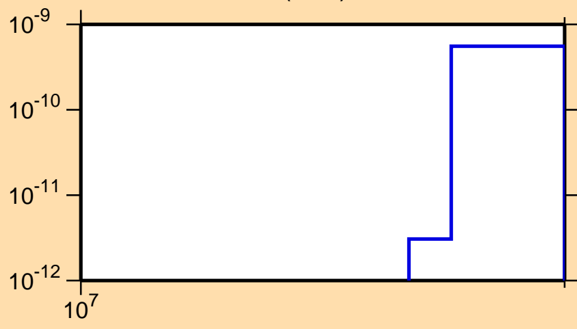
\sigma vs. E for ^{180}\text{Tl}(n,nt)
