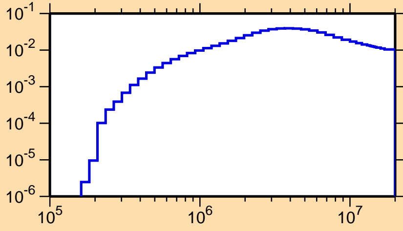
\sigma vs. E for ^{180}\text{Tl}(n,n_1)
