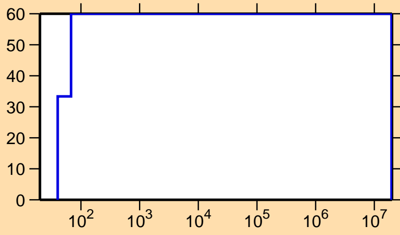
\Delta\sigma/\sigma vs. E for ^{180}\text{Tl}(n,\gamma)
