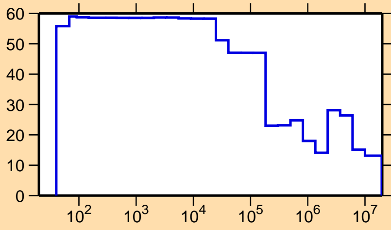
\Delta\sigma/\sigma vs. E for ^{180}\text{Tl}(n,el.)
