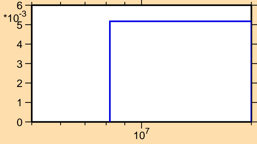
\sigma vs. E for ^{180}\text{Tl}(n,2n\alpha)
