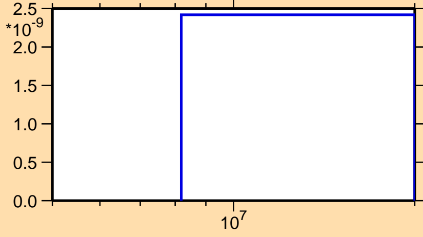
\sigma vs. E for ^{180}\text{Tl}(\text{mt } 34)
