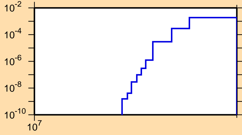
\sigma vs. E for ^{181}\text{Tl}(n,2np)
