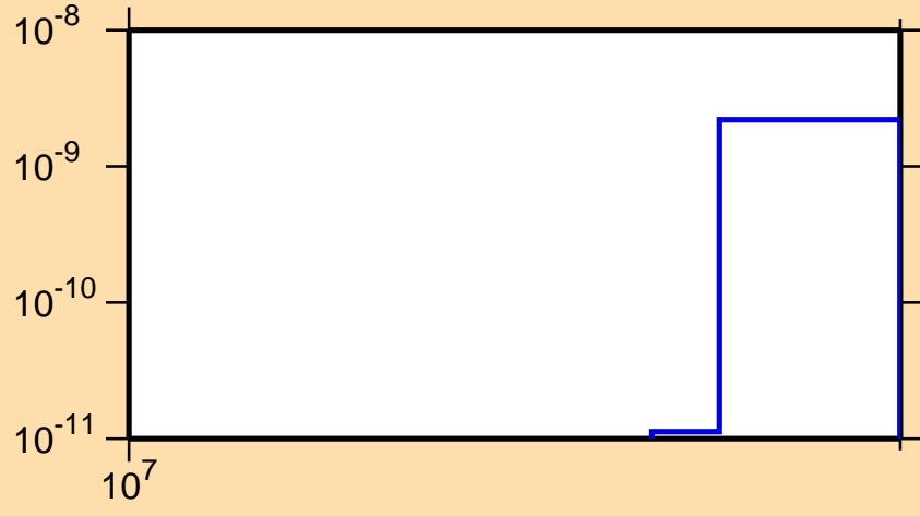
\sigma vs. E for ^{181}\text{Tl}(n,nt)
