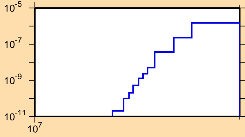
\sigma vs. E for ^{181}\text{Tl}(n,\text{nd})
