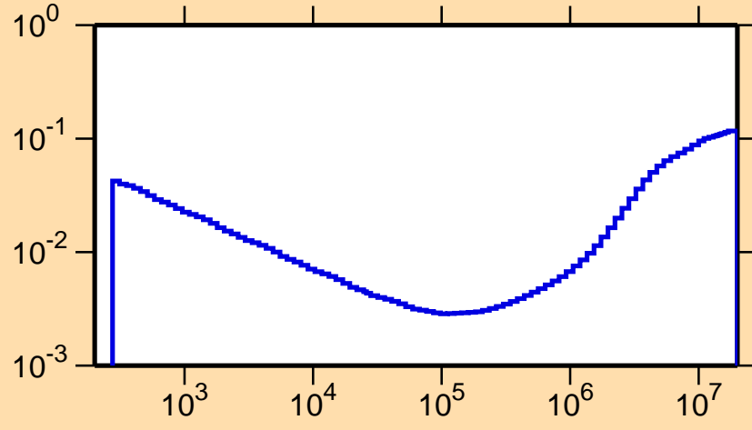
\sigma vs. E for ^{181}\text{Tl}(n,p\alpha)
