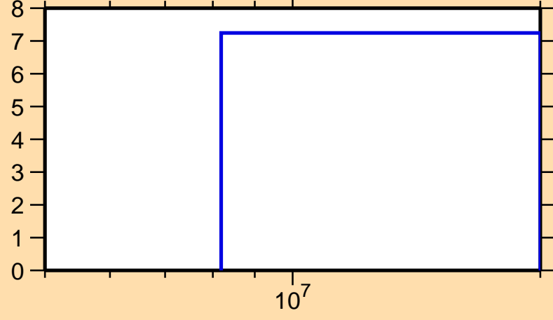
\Delta\sigma/\sigma vs. E for ^{181}\text{Tl}(n,\text{nonel.})
