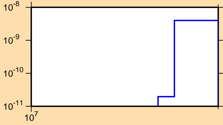
\sigma vs. E for ^{182}\text{Tl}(n,nt)
