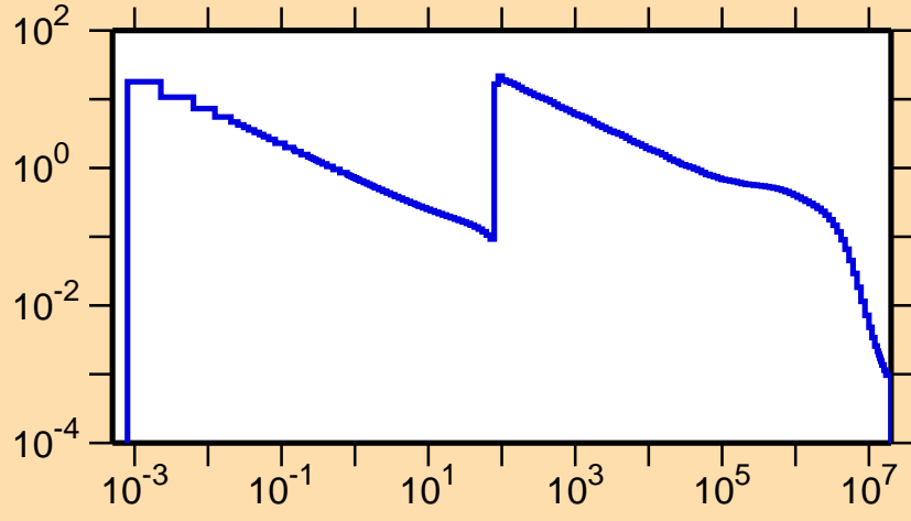
\sigma vs. E for ^{182}\text{Tl}(n,\gamma)
