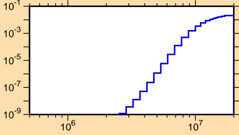
\sigma vs. E for ^{182}\text{Tl}(n,d)
