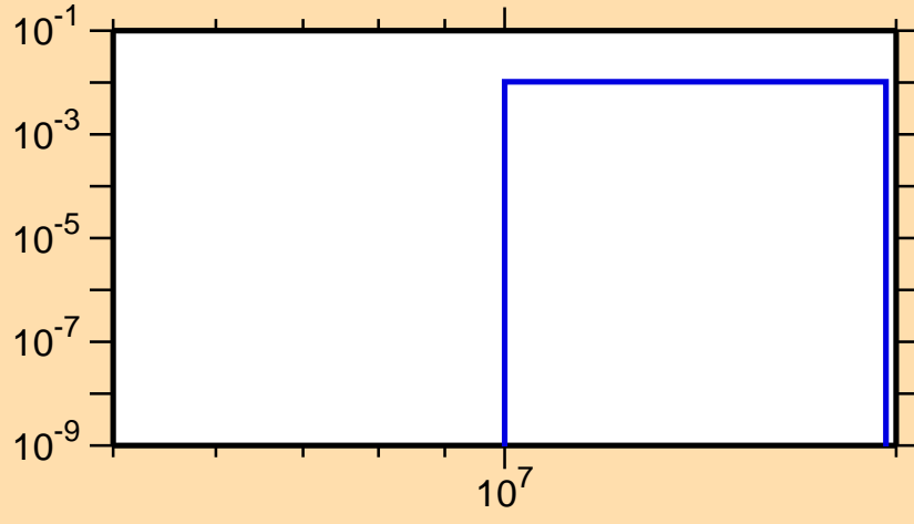
\sigma vs. E for ^{182}\text{Tl}(n,2n\alpha)
