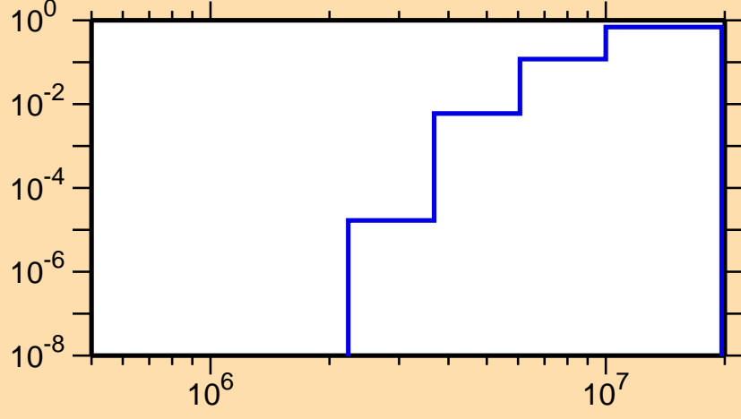
\sigma vs. E for ^{182}\text{Tl}(n,np)
