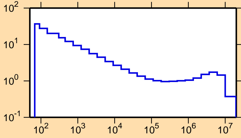
\sigma vs. E for ^{182}\text{Tl}(n,p)
