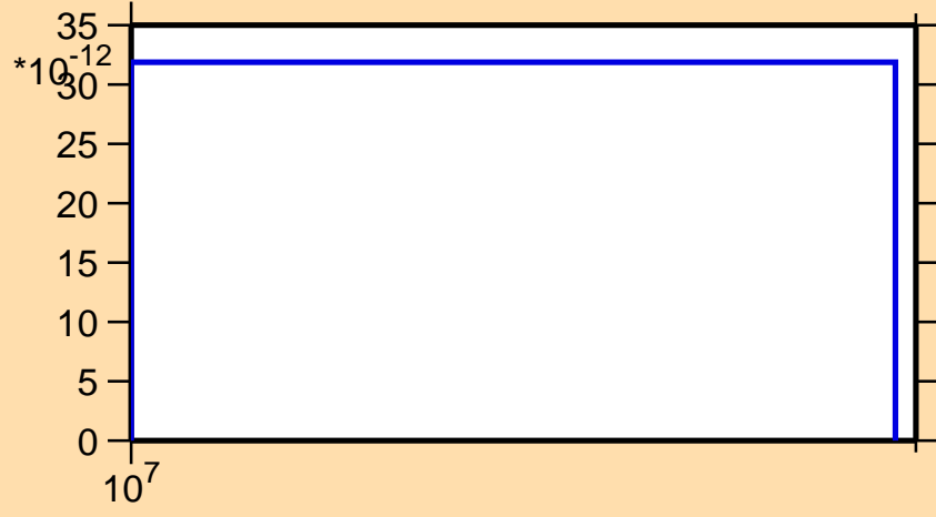
\sigma vs. E for ^{182}\text{Tl}(n,nt)
