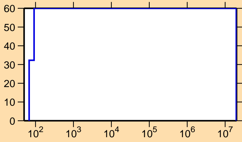
\Delta\sigma/\sigma vs. E for ^{182}\text{Tl}(n,p)
