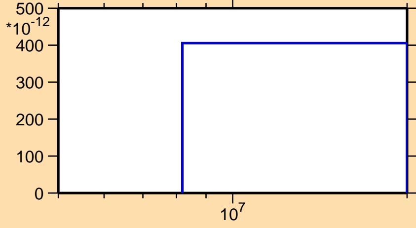
\sigma vs. E for ^{182}\text{Tl} (mt 34)
