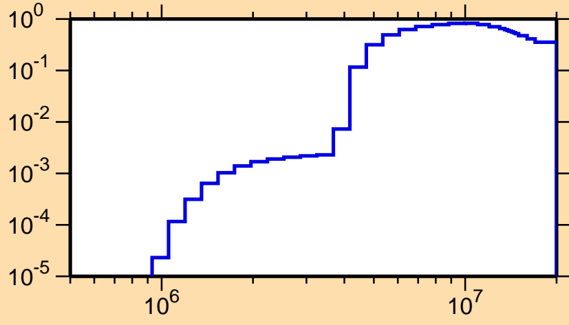
\sigma vs. E for ^{183}\text{Tl}(n,n\text{cont.})
