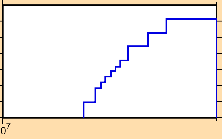
\sigma vs. E for ^{183}\text{Tl}(n,\text{nd})
