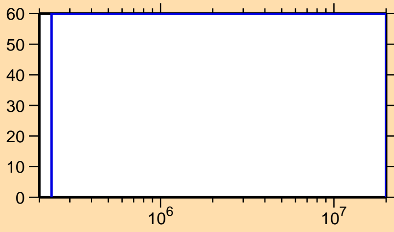
\Delta\sigma/\sigma vs. E for ^{183}\text{Tl}(n,n_1)
