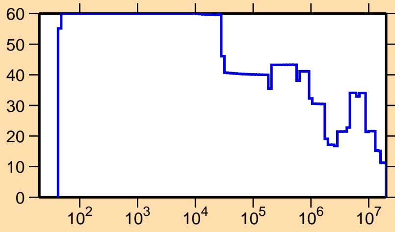
\Delta\sigma/\sigma vs. E for ^{183}\text{Tl}(n,el.)
