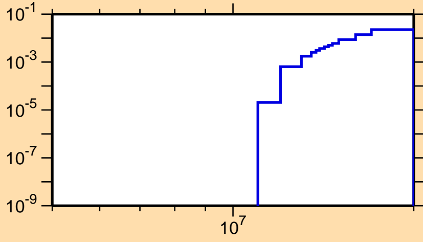
\sigma vs. E for ^{183}\text{Tl}(n,2n\alpha)
