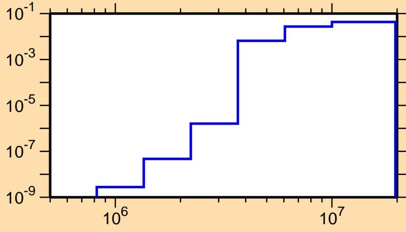
\sigma vs. E for ^{183}\text{Tl}(n,n\alpha)
