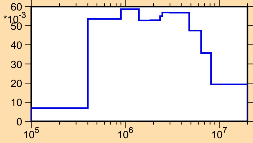
\sigma vs. E for ^{183}\text{Tl}(n,n_1)
