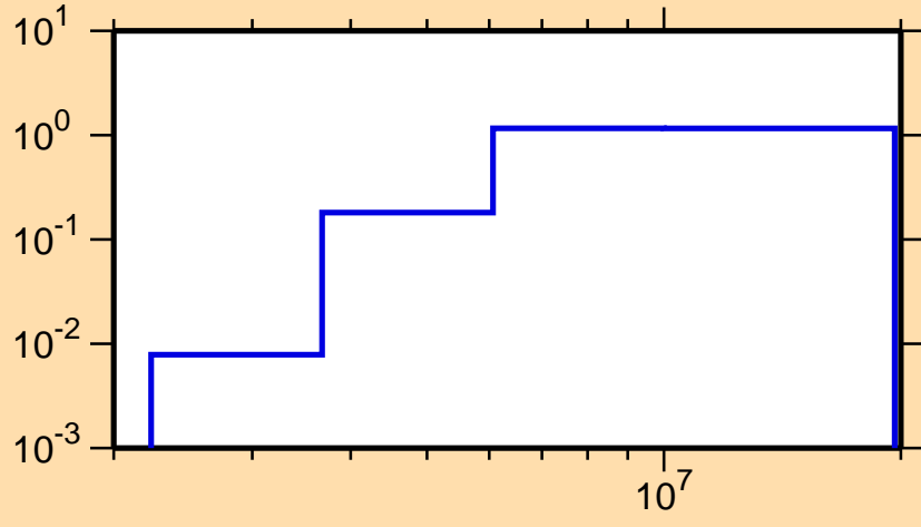
\sigma vs. E for ^{185}\text{Tl}(n,n\text{cont.})
