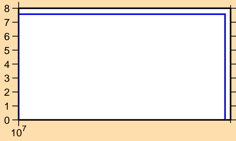
\Delta\sigma/\sigma vs. E for ^{185}\text{Tl}(n,\text{tot.})
