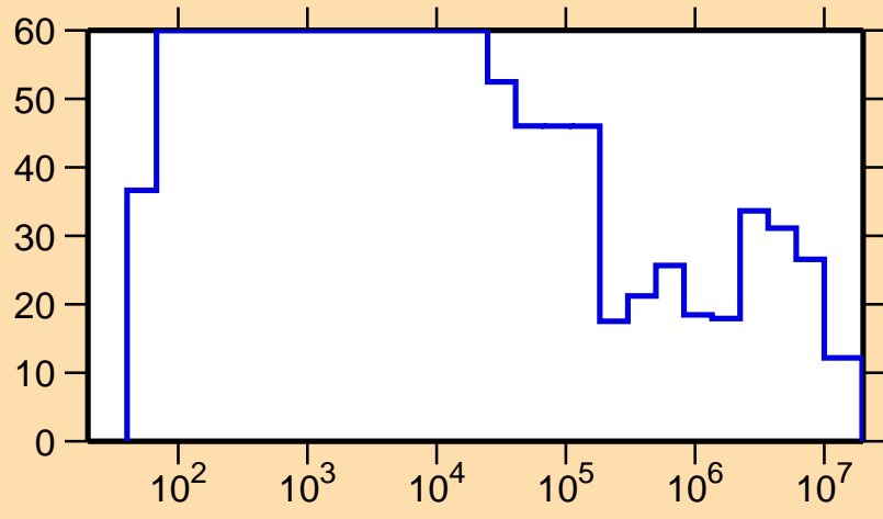
\Delta\sigma/\sigma vs. E for ^{185}\text{Tl}(n,el.)
