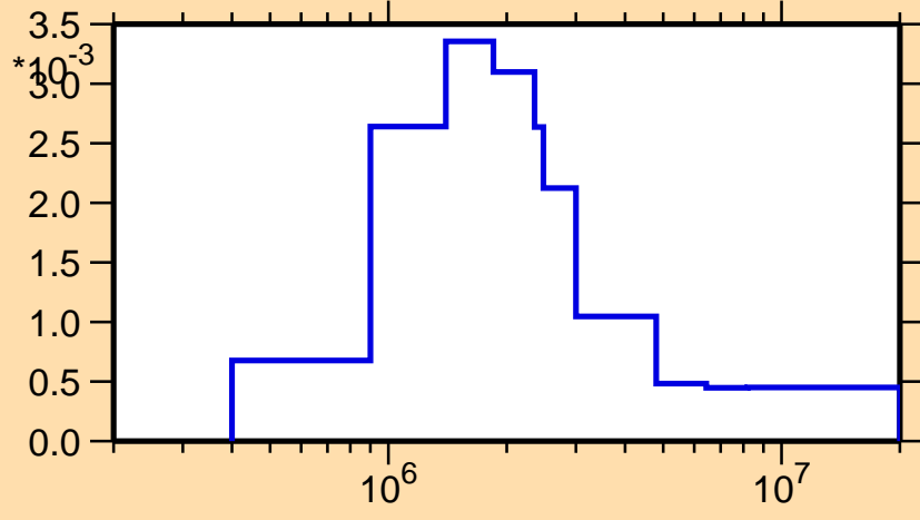
\sigma vs. E for ^{185}\text{Tl}(n,n_3)
