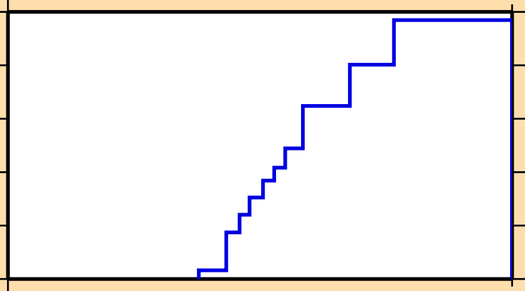
\sigma vs. E for ^{185}\text{Tl}(n,\text{nd})
