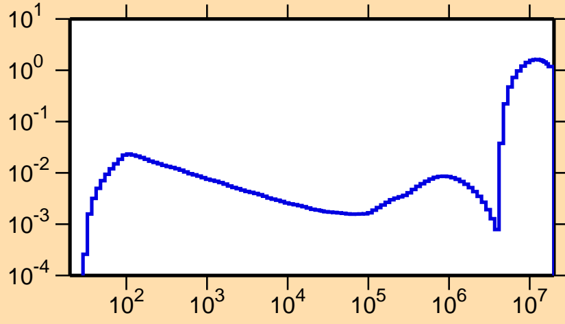
\sigma vs. E for ^{185}\text{Tl}(n,\text{inel.})
