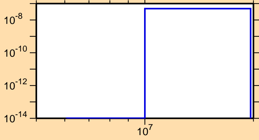
\sigma vs. E for ^{185}\text{Tl}(n,pd)
