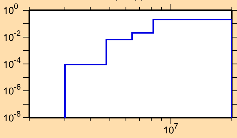
\sigma vs. E for ^{185}\text{Tl}(n,np)
