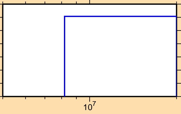
\sigma vs. E for ^{185}\text{Tl}(n,nd)
