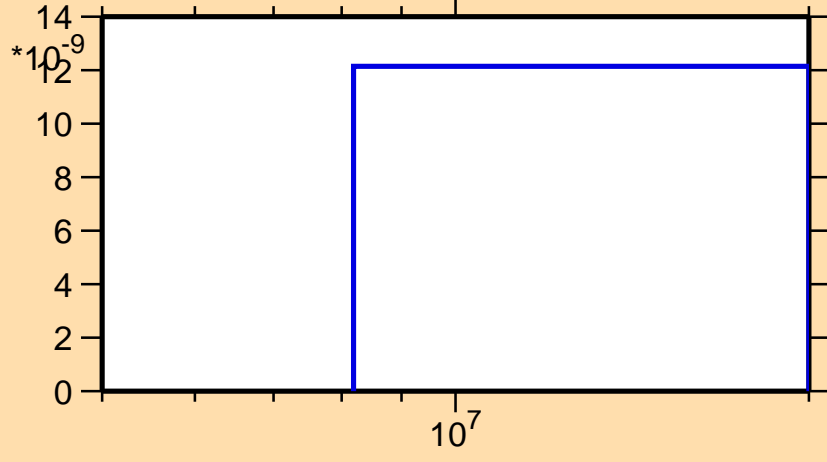
\sigma vs. E for ^{185}\text{Tl}(n,nd)
