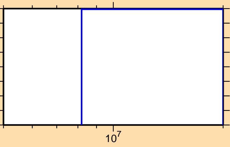
\sigma vs. E for ^{185}\text{Tl}(n,\text{pd})
