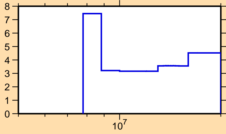
\Delta\sigma/\sigma vs. E for ^{186}\text{Tl}(n,\text{tot.})
