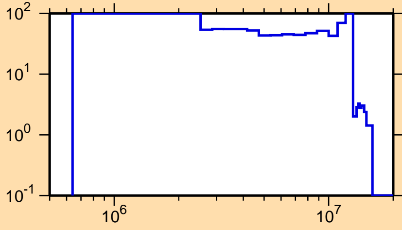
\Delta\sigma/\sigma vs. E for ^{186}\text{Tl}(n,n_1)
