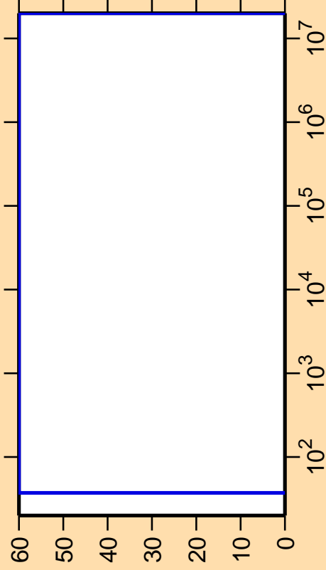
\Delta\sigma/\sigma vs. E for ^{186}\text{Tl}(n,\alpha)
