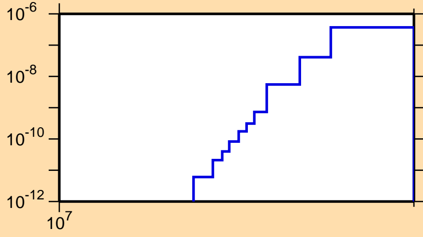
\sigma vs. E for ^{186}\text{Tl}(n,\text{pt})
