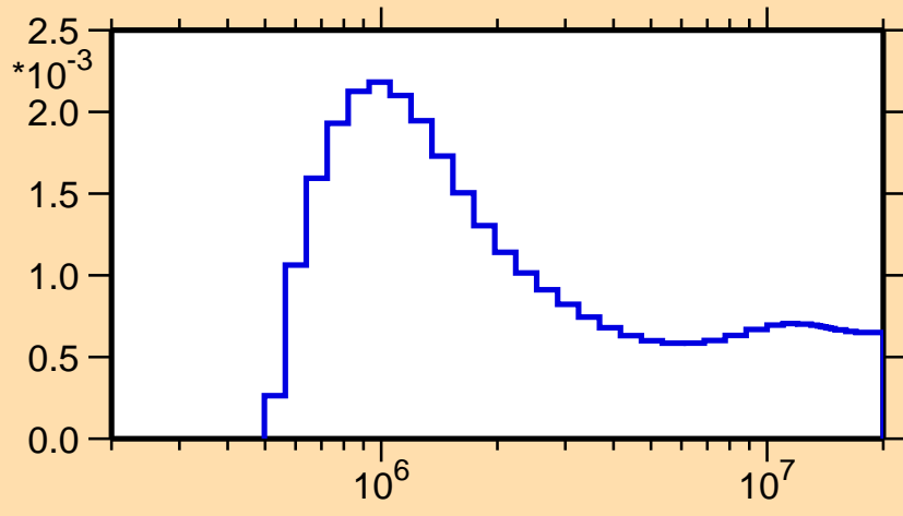
\sigma vs. E for ^{186}\text{Tl}(n,n_4)
