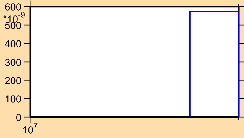
\sigma vs. E for ^{186}\text{Tl}(n,3n)
