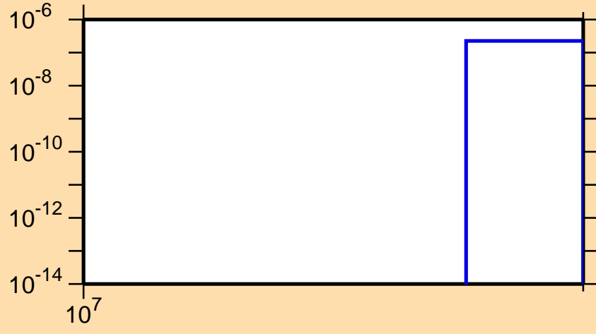
\sigma vs. E for ^{186}\text{Tl}(n,3n\alpha)
