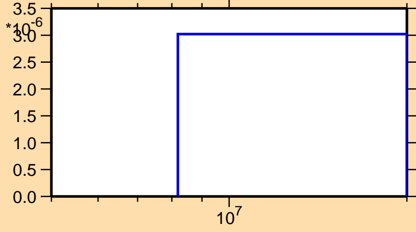
\sigma vs. E for ^{186}\text{Tl}(n,nd)
