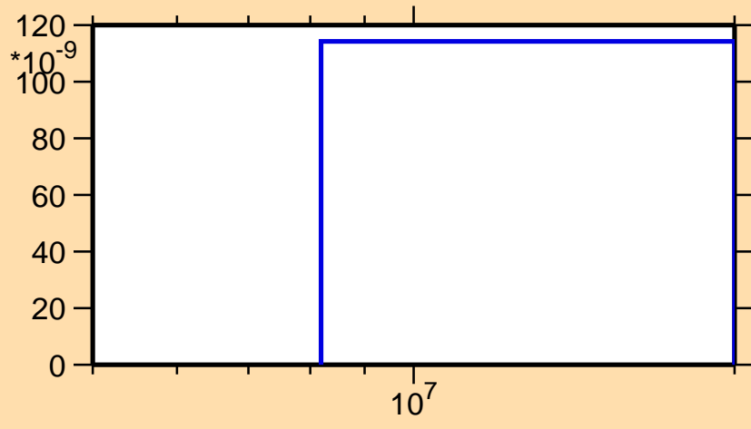
\sigma vs. E for ^{186}\text{Tl}(n,\text{pd})
