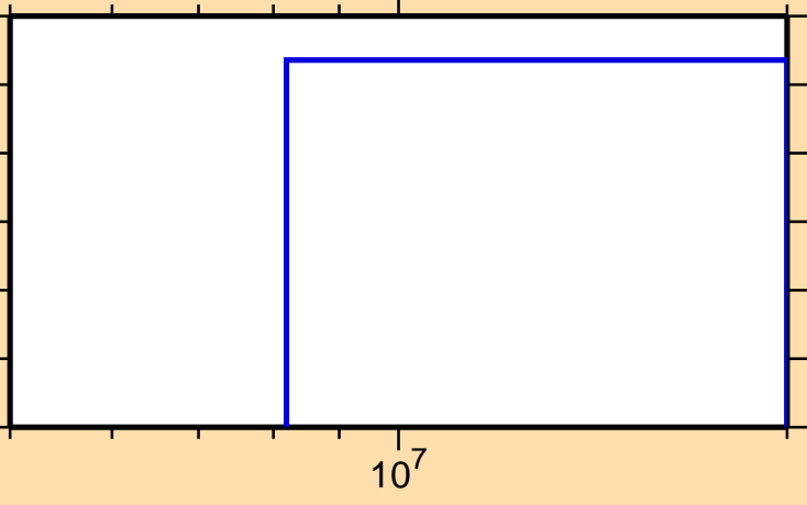
\sigma vs. E for ^{186}\text{Tl}(n,\text{pt})
