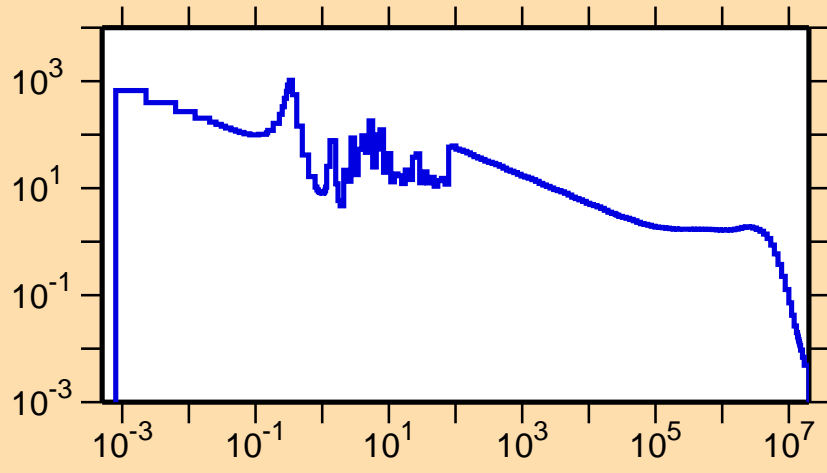
\sigma vs. E for ^{187}\text{Tl}(n,\gamma)
