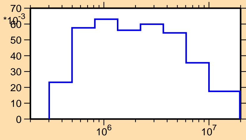
\sigma vs. E for ^{187}\text{Tl}(n,n_1)
