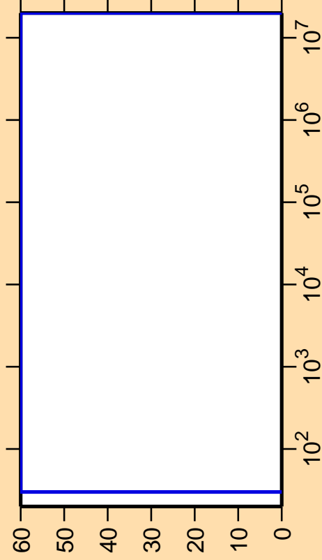
\Delta\sigma/\sigma vs. E for ^{187}\text{Tl}(n,p\alpha)
