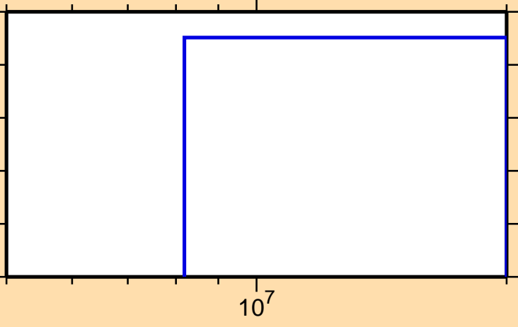
\sigma vs. E for ^{187}\text{Tl}(n,2n\alpha)
