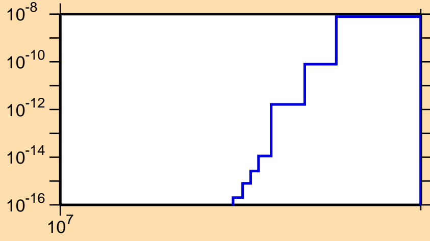
\sigma vs. E for ^{187}\text{Tl}(n,nt)
