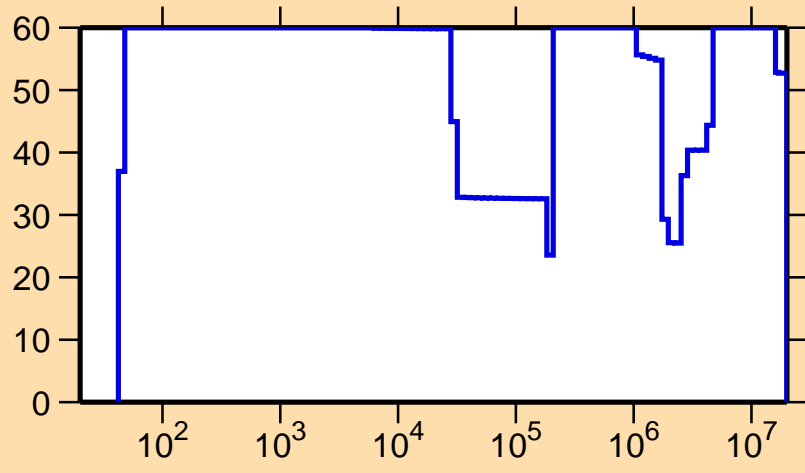
\Delta\sigma/\sigma vs. E for ^{187}\text{Tl}(n,el.)
