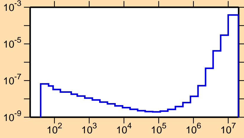
\sigma vs. E for ^{187}\text{Tl}(n,p\alpha)
