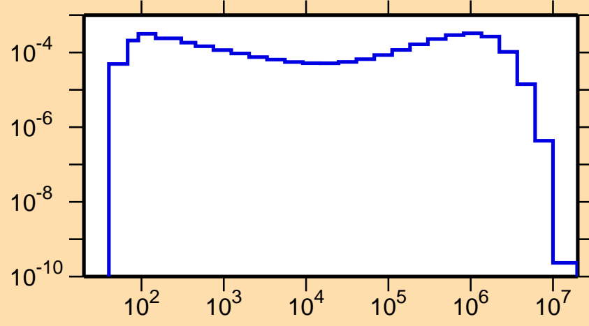
\sigma vs. E for ^{187}\text{Tl}(n,n_1)
