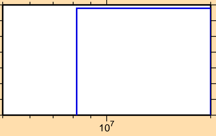
\sigma vs. E for ^{187}\text{Tl}(n,\text{nd})
