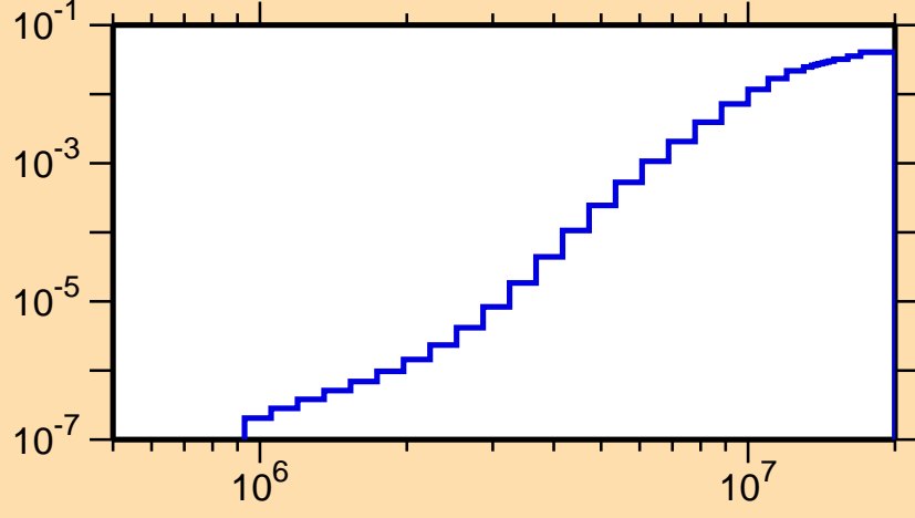
\sigma vs. E for ^{188}\text{Tl}(n,n\alpha)
