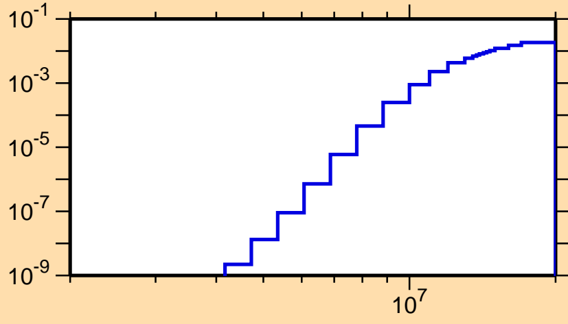
\sigma vs. E for ^{188}\text{Tl}(n,d)
