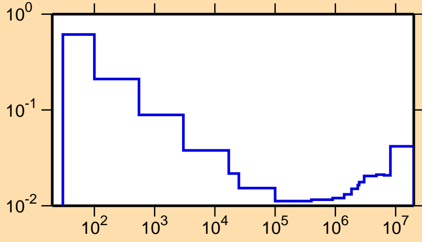
\sigma vs. E for ^{188}\text{Tl}(n,\alpha)
