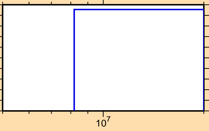
\sigma vs. E for ^{188}\text{Tl}(n,nt)
