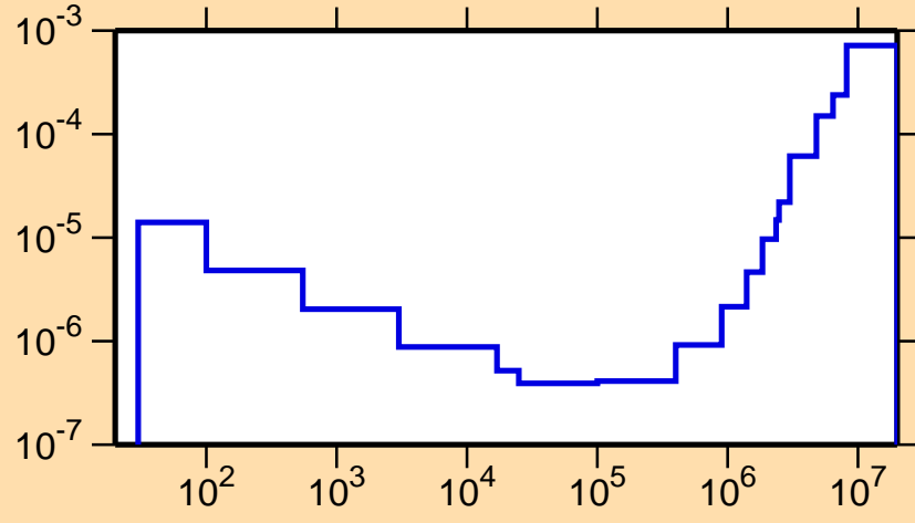
\sigma vs. E for ^{188}\text{Tl}(n,p\alpha)
