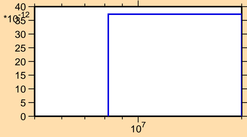
\sigma vs. E for ^{188}\text{Tl} (mt 34)
