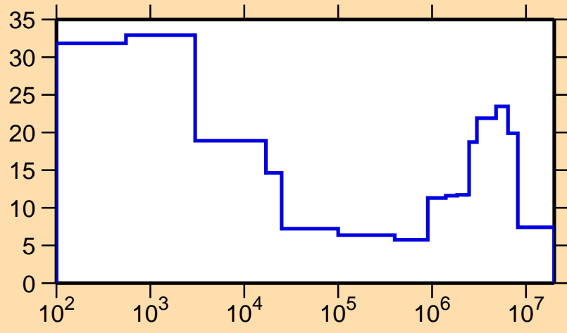
\Delta\sigma/\sigma vs. E for ^{189}\text{Tl}(n,el.)
