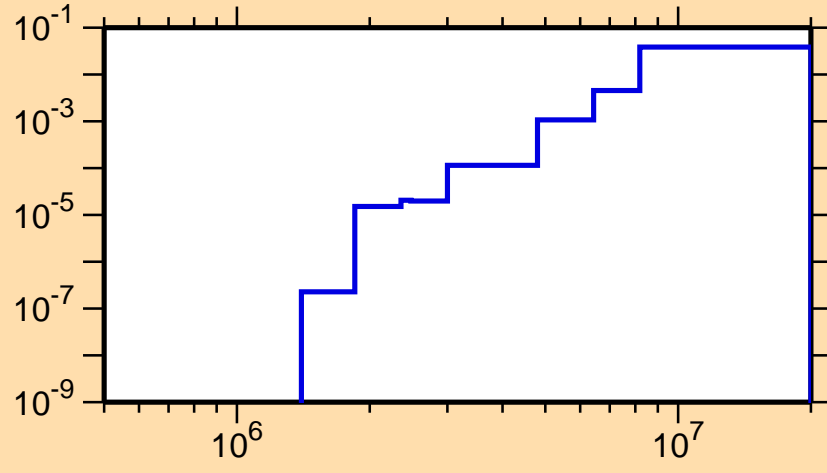
\sigma vs. E for ^{189}\text{Tl}(n,n\alpha)
