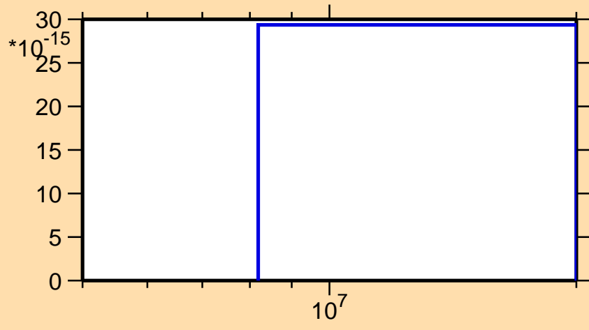
\sigma vs. E for ^{189}\text{Tl} (mt 34)
