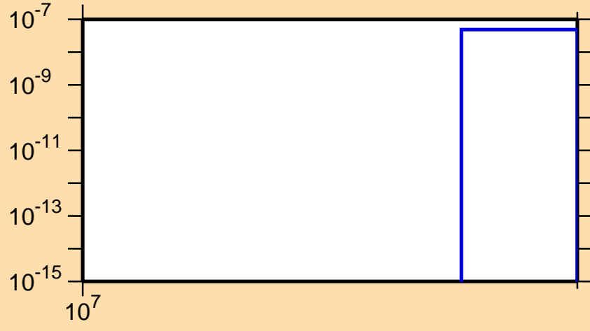
\sigma vs. E for ^{189}\text{Tl}(n,3n\alpha)
