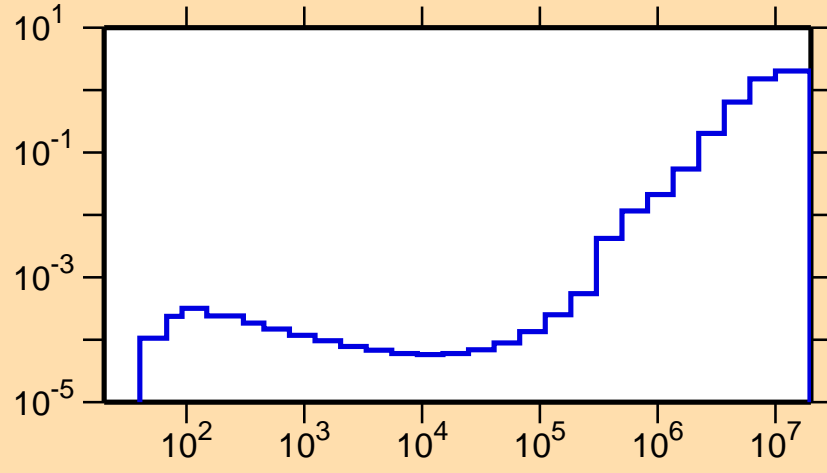
\sigma vs. E for ^{189}\text{Tl}(n,\text{inel.})
