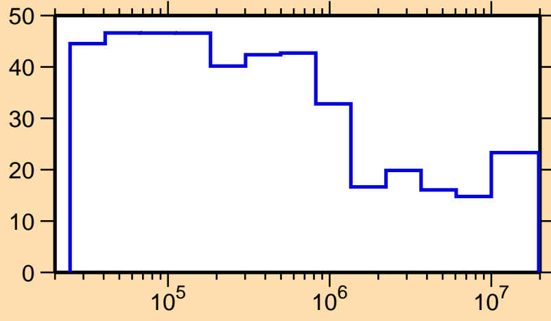
\Delta\sigma/\sigma vs. E for ^{189}\text{Tl}(n,\text{tot.})
