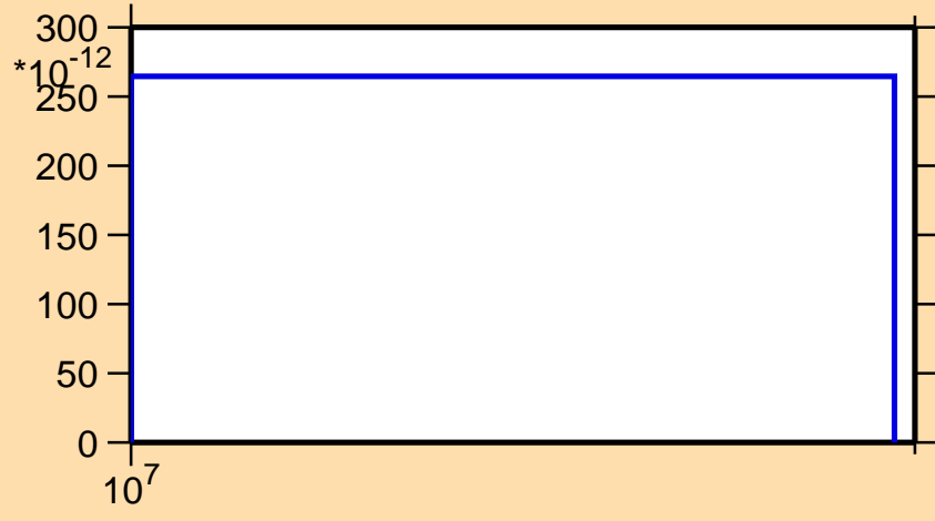
\sigma vs. E for ^{189}\text{Tl}(n,3n\alpha)
