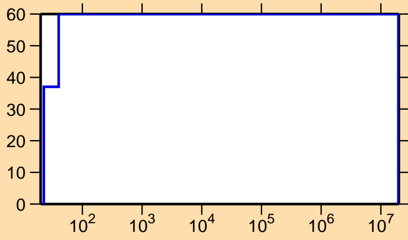
\Delta\sigma/\sigma vs. E for ^{189}\text{Tl}(n,\gamma)
