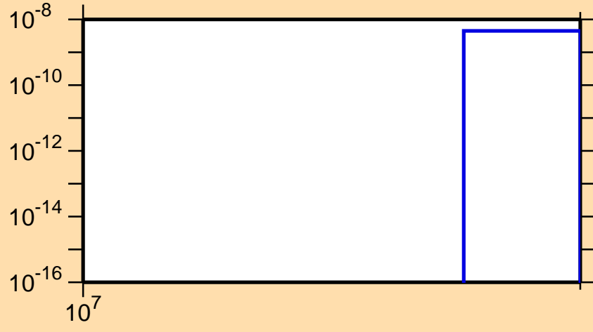
\sigma vs. E for ^{190}\text{Tl}(n,3n\alpha)
