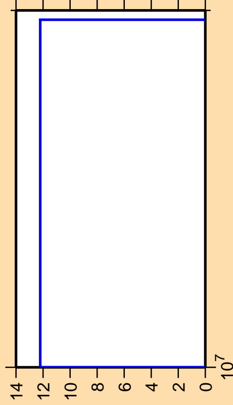
\Delta\sigma/\sigma vs. E for ^{190}\text{Tl} (mt 34)
