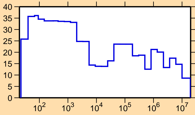
\Delta\sigma/\sigma vs. E for ^{190}\text{Tl}(n,el.)
