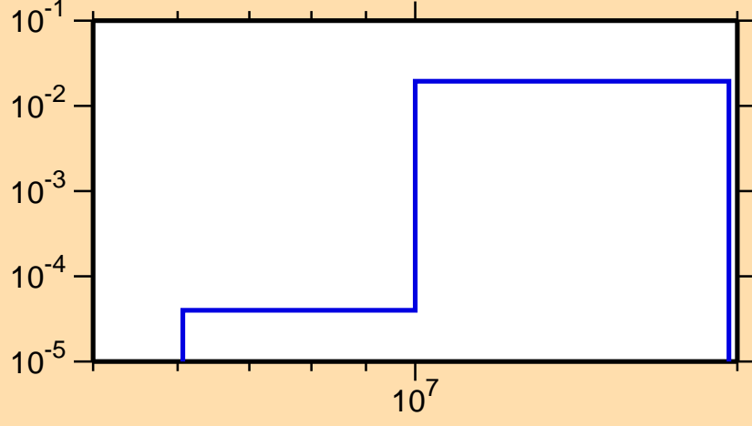
\sigma vs. E for ^{190}\text{Tl}(n,2n\alpha)
