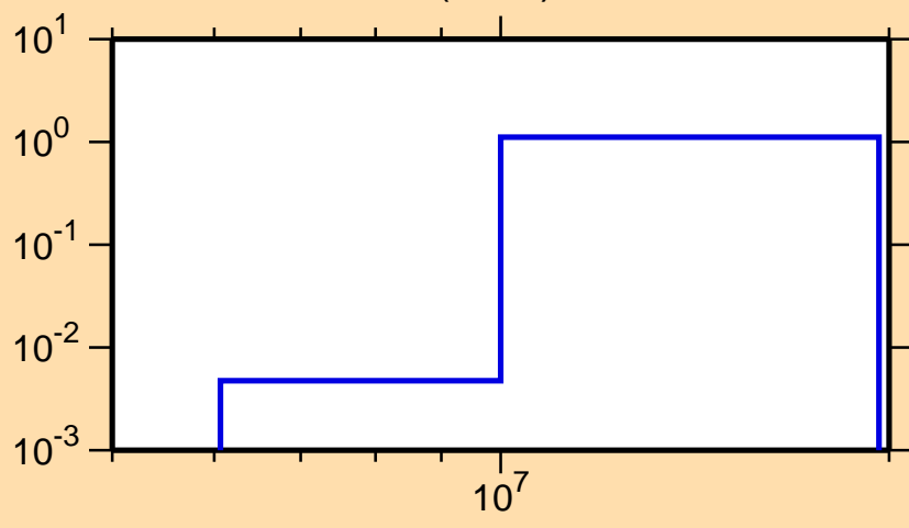
\sigma vs. E for ^{190}\text{Tl}(n,2n)
