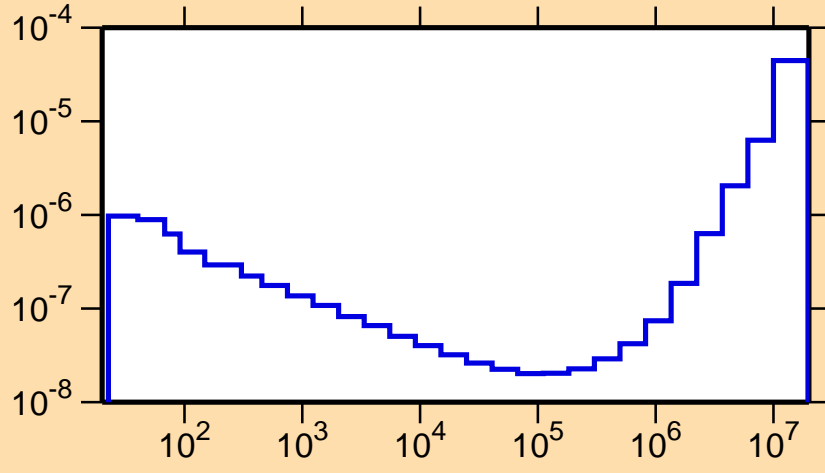
\sigma vs. E for ^{190}\text{Tl}(n,p\alpha)
