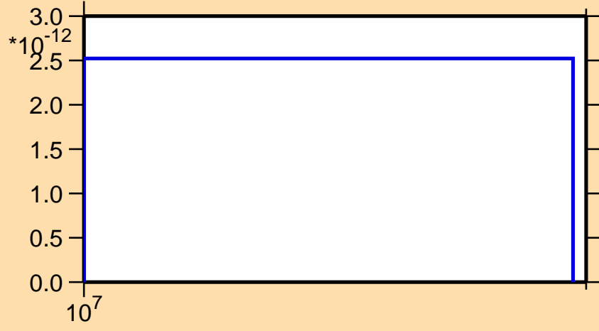
\sigma vs. E for ^{190}\text{Tl} (mt 34)
