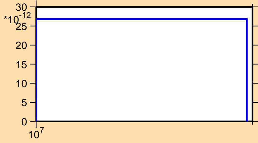
\sigma vs. E for ^{190}\text{Tl}(n,3n\alpha)
