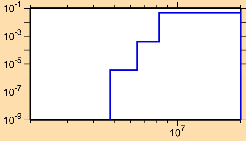
\sigma vs. E for ^{190}\text{Tl}(n,np)
