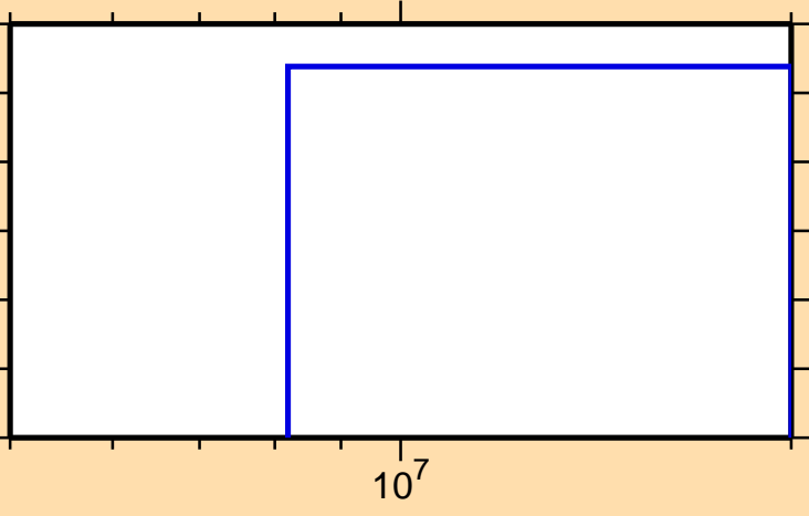
\sigma vs. E for ^{190}\text{Tl}(n,2np)
