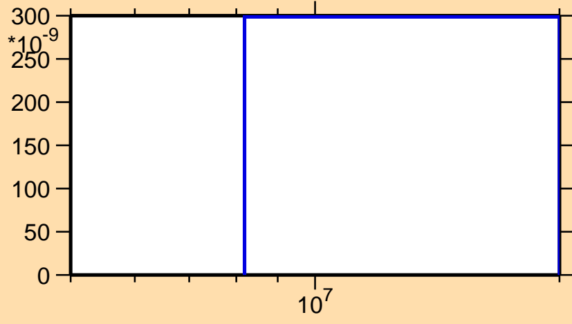
\sigma vs. E for ^{190}\text{Tl}(n,\text{nd})
