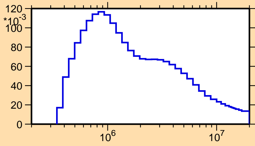
\sigma vs. E for ^{191}\text{Tl}(n,n_1)
