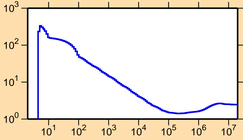
\sigma vs. E for ^{191}\text{Tl}(n,\text{nonel.})
