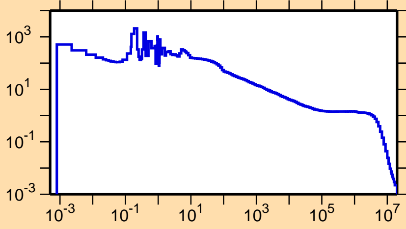
\sigma vs. E for ^{191}\text{Tl}(n,\gamma)
