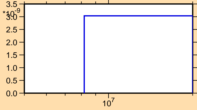
\sigma vs. E for ^{191}\text{Tl}(n,3n\alpha)
