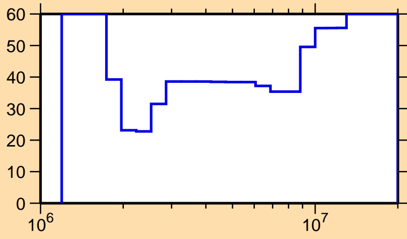
\Delta\sigma/\sigma vs. E for ^{192}\text{Tl}(n,n\text{cont.})
