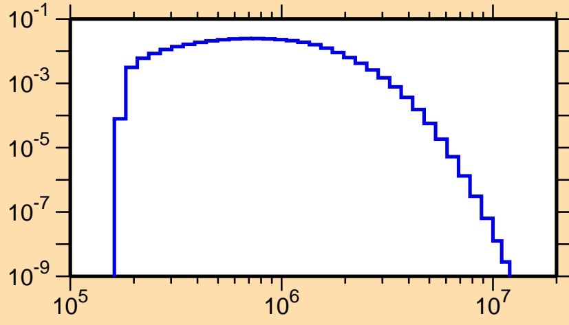
\sigma vs. E for ^{192}\text{Tl}(n,n_3)
