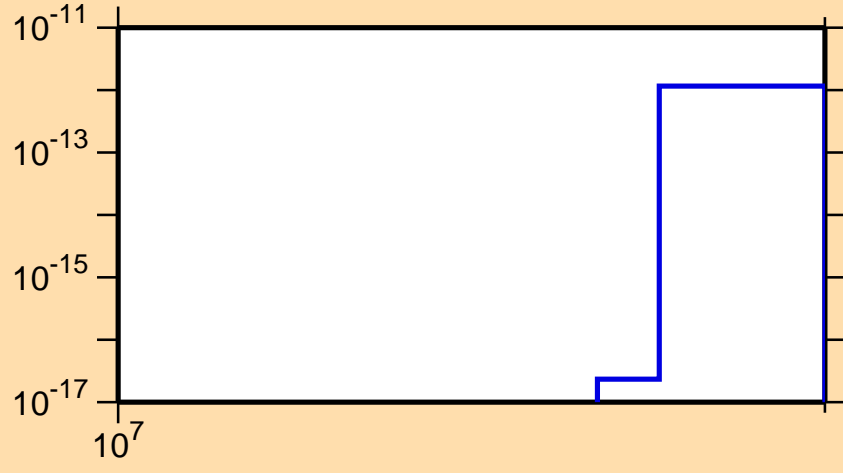
\sigma vs. E for ^{192}\text{Tl}(n,3n\alpha)
