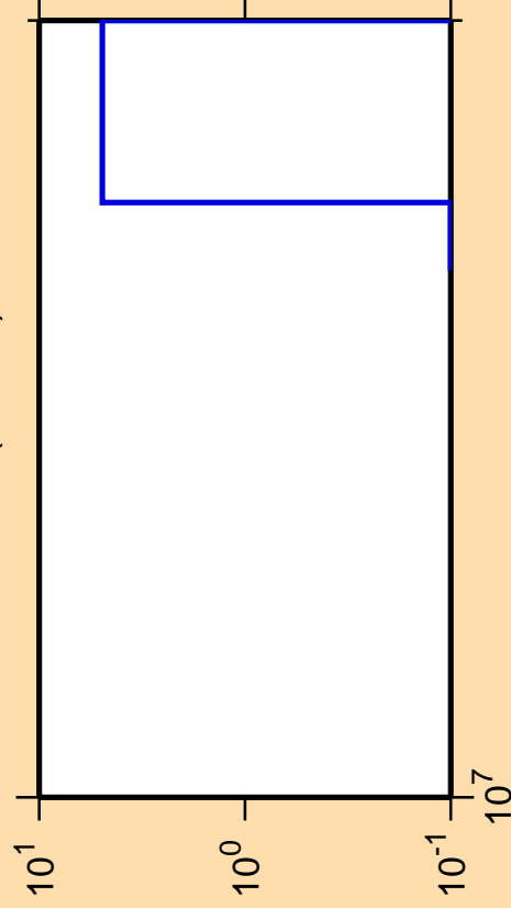
\Delta\sigma/\sigma vs. E for ^{192}\text{Tl}(n,3n\alpha)
