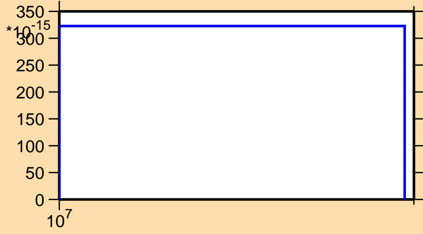
\sigma vs. E for ^{192}\text{Tl} (mt 34)
