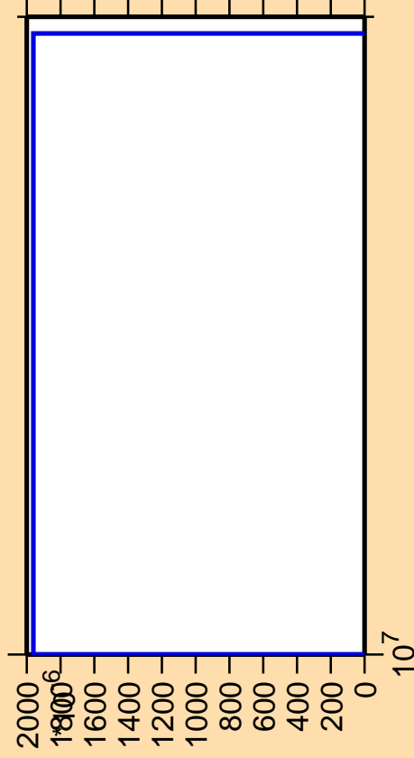
\Delta\sigma/\sigma vs. E for ^{192}\text{Tl}(n,3n\alpha)
