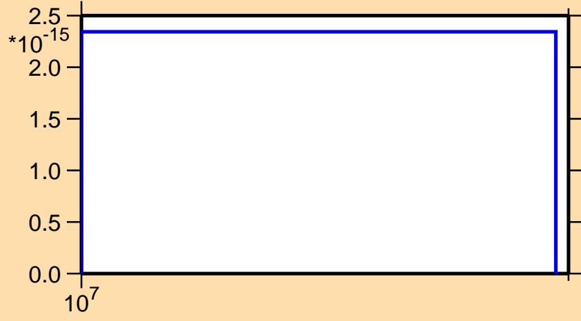
\sigma vs. E for ^{192}\text{Tl}(n,3n\alpha)
