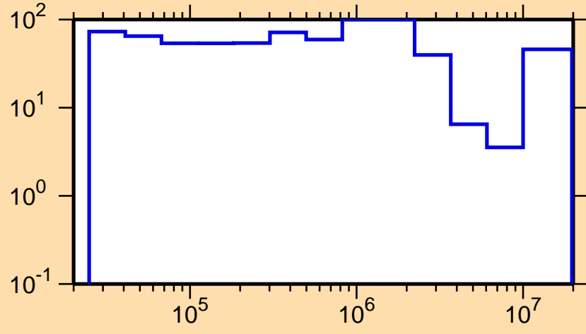
\Delta\sigma/\sigma vs. E for ^{192}\text{Tl}(n,ncont.)
