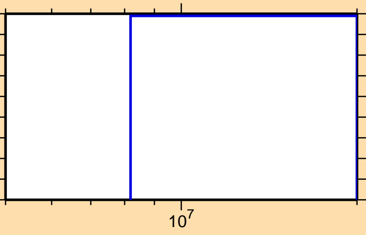
\sigma vs. E for ^{192}\text{Tl}(n,nd)
