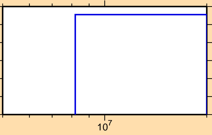
\sigma vs. E for ^{192}\text{Tl}(n,2n\alpha)
