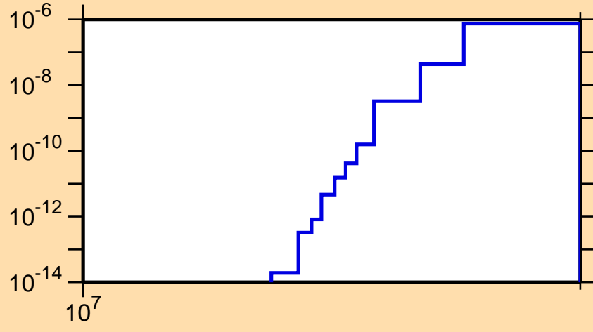
\sigma vs. E for ^{193}\text{Tl}(n,nd)
